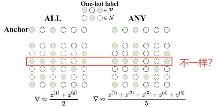
Figure 1: Illustration for ALL and ANY method. Each row represents one sample's label, where the first row is the anchor and the following ones are samples in \mathcal{A} , here |\mathcal{A}| = 6 . Each sample's label is denoted in a one-hot form where the green circle means 1. The row with circles plotted with dotted line means that the corresponding sample is in the negative set \mathcal{N} , otherwise the sample is in the positive set \mathcal{P} .
