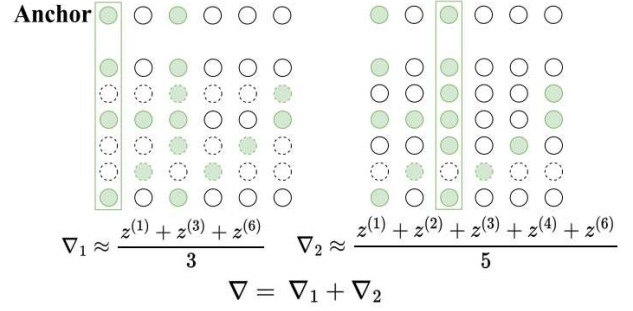
Figure 2: The proposed MulSupCon loss function. We consider each label separately and form multiple positive sets for one anchor sample. The positive sets for the anchor is \mathcal{P}_1 = \{1, 3, 6\} , \mathcal{P}_3 = \{1, 2, 3, 4, 6\} , suppose the anchor's label is \mathbf{y} = \{1, 3\} .
